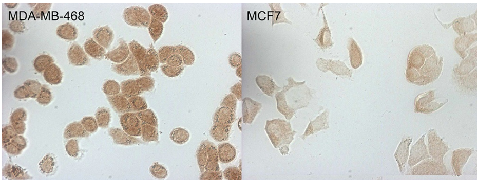
Immunocytochemistry staining of MDA-MB-468 cells using anti-CDKN2A mouse monoclonal antibody ([TA805398]). The right is MCF7 cells as negative control (1:100).
