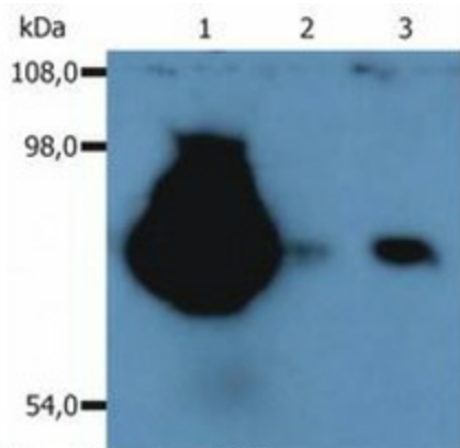
Fig. 1. Western Blotting
