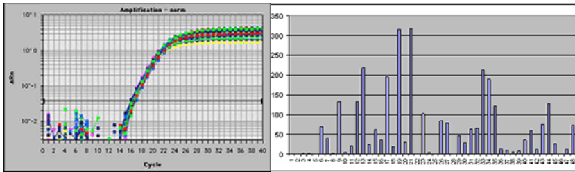
A Human Thyroid Cancer real time PCR Gene Expression panel was used in real-time PCR. The beta-actin contents in the 48 human cDNAs were detected user SYBR Green I protocol in PE7700.
