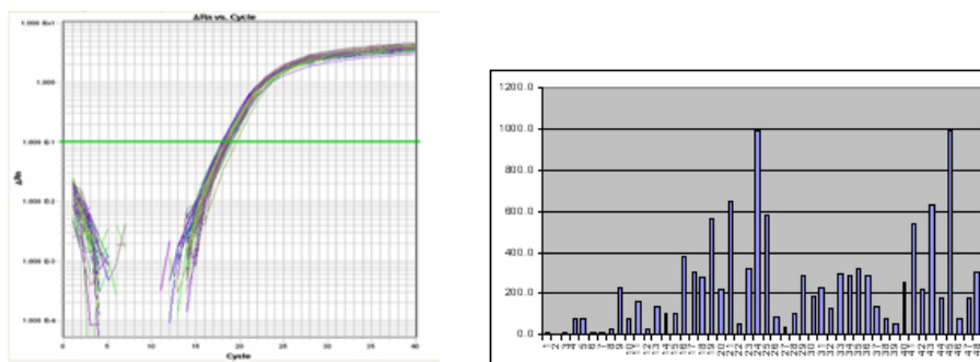
Left: EDRT102 panel was used for beta-actin amplification showing normalization of the cDNA. Right: Expression level of a control gene, survivin, was plotted. Both assays were performed using SYBR Green I Protocol in an ABI7900HT instrument.
