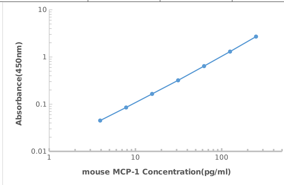
Representative standard curve for MCP-1 ELISA.
