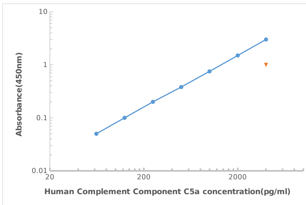
Representative standard curve for Complement Component C5a ELISA.
