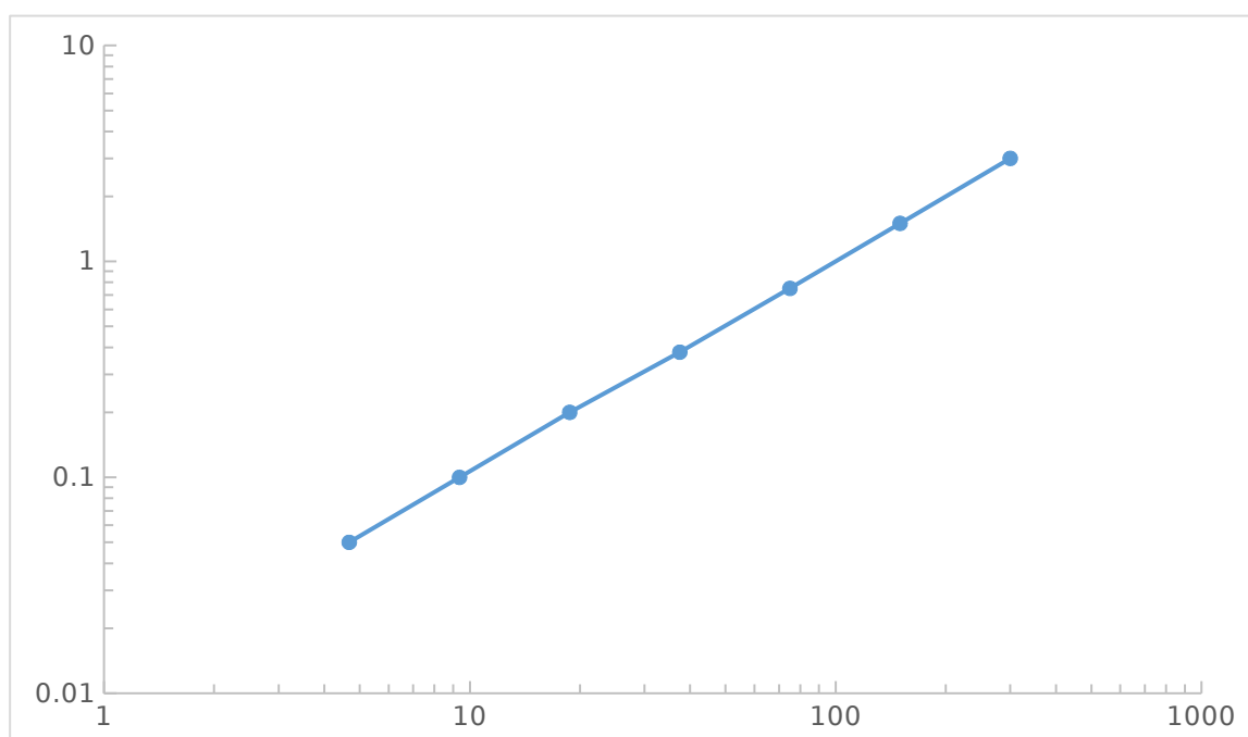
Representative standard curve for GM-CSF ELISA.
