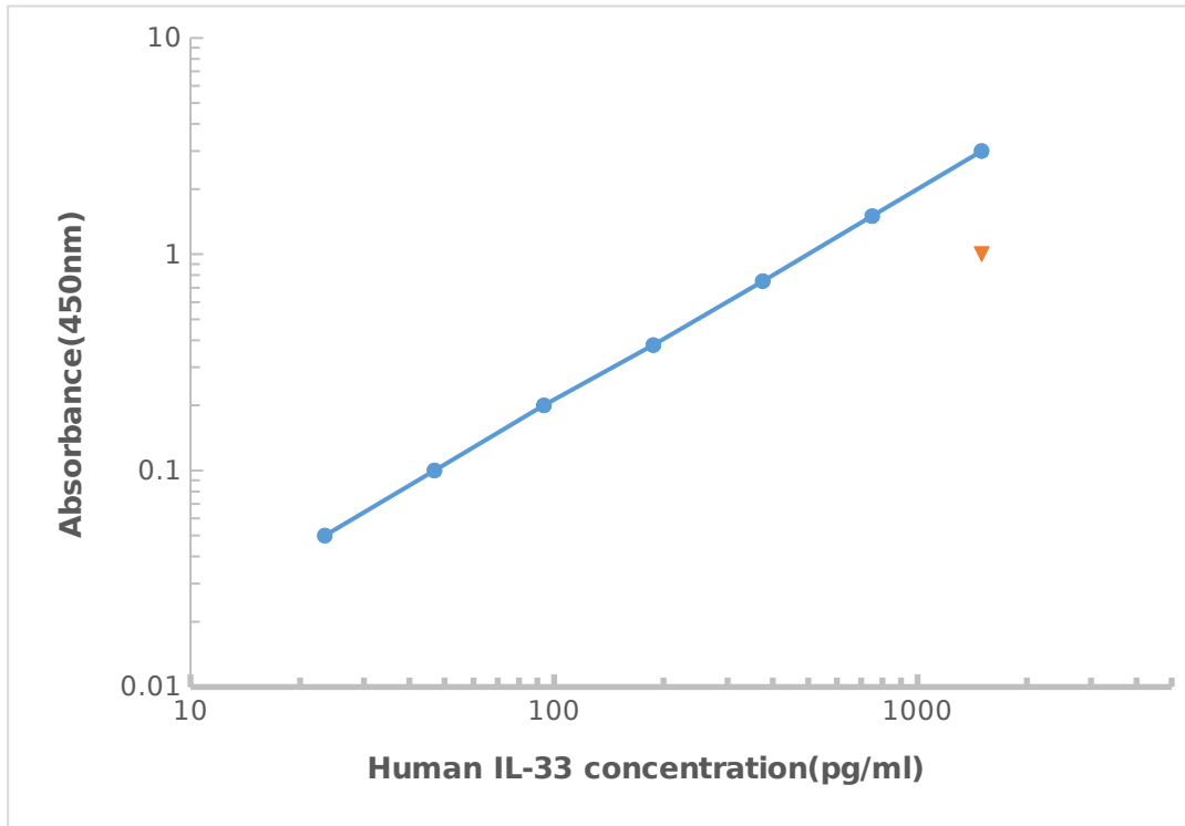
Representative standard curve for IL-33 ELISA.
