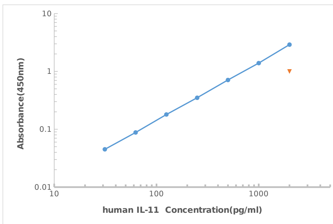
Representative standard curve for IL-11 ELISA.
