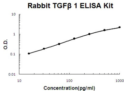
Rabbit TGF beta 1 ELISA Kit standard curve
