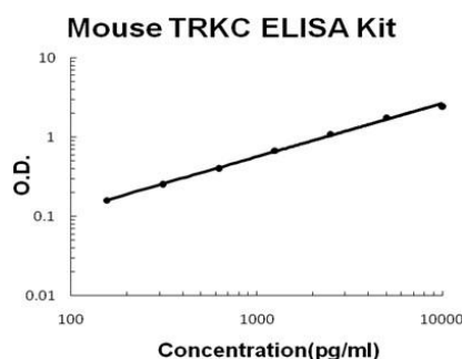
Mouse TRKC ELISA Kit standard curve
