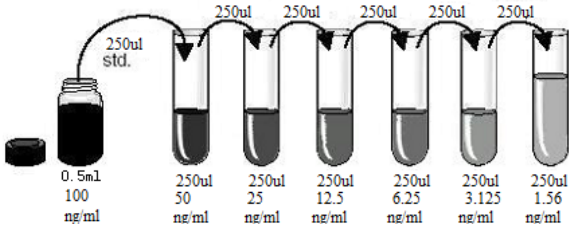
Figure 2: Preparation of PBEF/Visfatin standard dilutions
