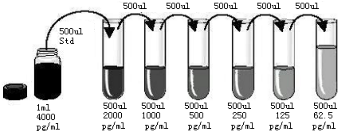
Figure 2: Preparation of APO-1/FAS standard dilutions
