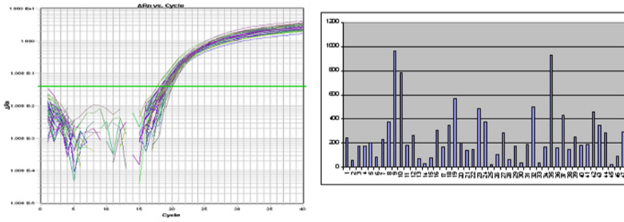
Left: CCRT102 panel was used for beta-actin amplification showing normalization of the cDNA. Right: Expression level of a control gene, TNF-alpha was plotted. Both assays were performed using SYBR Green I Protocol in an ABI7900HT instrument.
