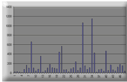
A Human Breast Cancer real time PCR Gene Expression panel was used in SYBR Green I based real-time PCR. The expression profile of the human Survivin (ACC# NM_001168) was detected using SYBR Green I protocol and performed in PE7700.
