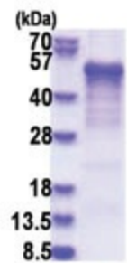
15% SDS-PAGE (3ug)
