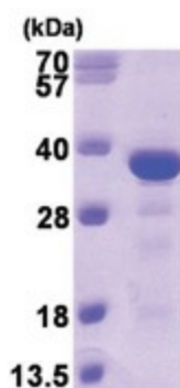
15% SDS-PAGE (3ug)
