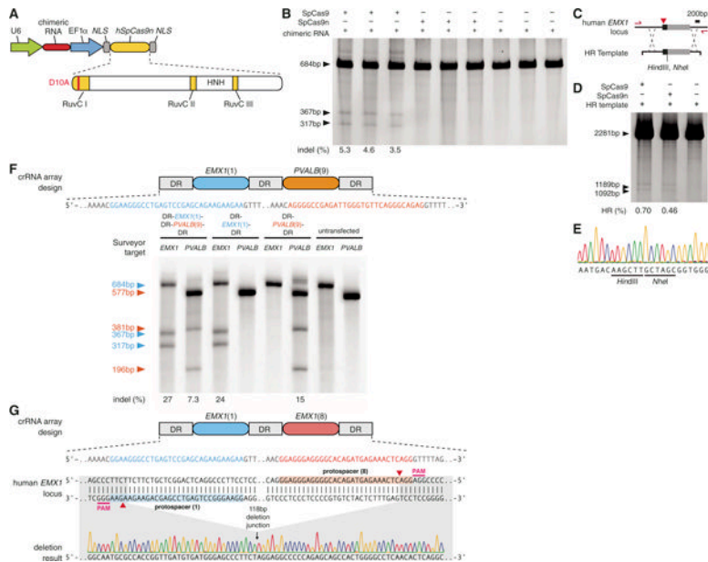
Fig. 4. Applications of Cas9 for homologous recombination and multiplex genome engineering. (A) Mutation of the RuvC I domain converts Cas9 into a nicking enzyme (SpCas9n). HNH, histidine-asparagine-histidine endonuclease domain. (B) Coexpression of EMX1 -targeting chimeric RNA with SpCas9 leads to indels, whereas SpCas9n does not ( N=3 ). (C) Schematic representation of the recombination strategy. A homology repair (HR) template is designed to insert restriction sites into EMX1 locus. Primers used to amplify the modified region are shown as red arrows. (D) Restriction fragment length polymorphism gel analysis. Arrows indicate fragments generated by HindIII digestion. (E) Example chromatogram showing successful recombination. (F) SpCas9 can facilitate multiplex genome modification by using a crRNA array that contains two spacers targeting EMX1 and PVALB . Schematic showing the design of the crRNA array (top). Both spacers mediate efficient protospacer cleavage (bottom). (G) SpCas9 can be used to achieve precise genomic deletion. Two spacers targeting EMX1 (top) mediated a 118-bp genomic deletion (bottom).
