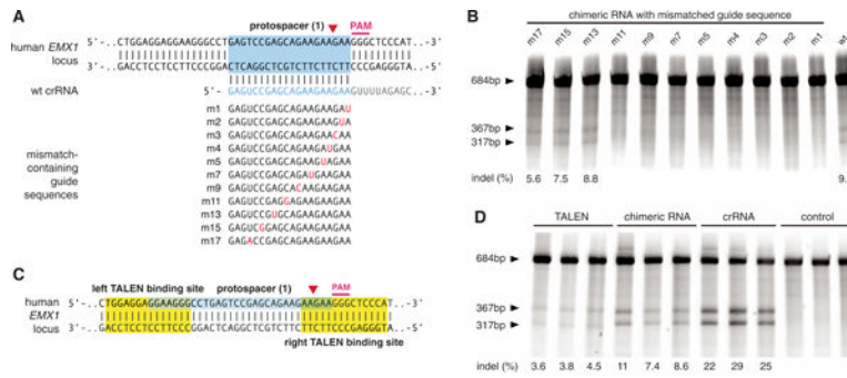
Fig. 3. Evaluation of the SpCas9 specificity and comparison of efficiency with TALENs. (A) EMX1 -targeting crRNAs with single point mutations were generated to evaluate the effects of spacer-protospacer mismatches. (B) SURVEYOR assay comparing the cleavage efficiency of different mutant chimeric RNAs. (C) Schematic showing the design of TALENs that target EMX1 . (D) SURVEYOR gel comparing the efficiency of TALEN and SpCas9 ( N = 3 ).
